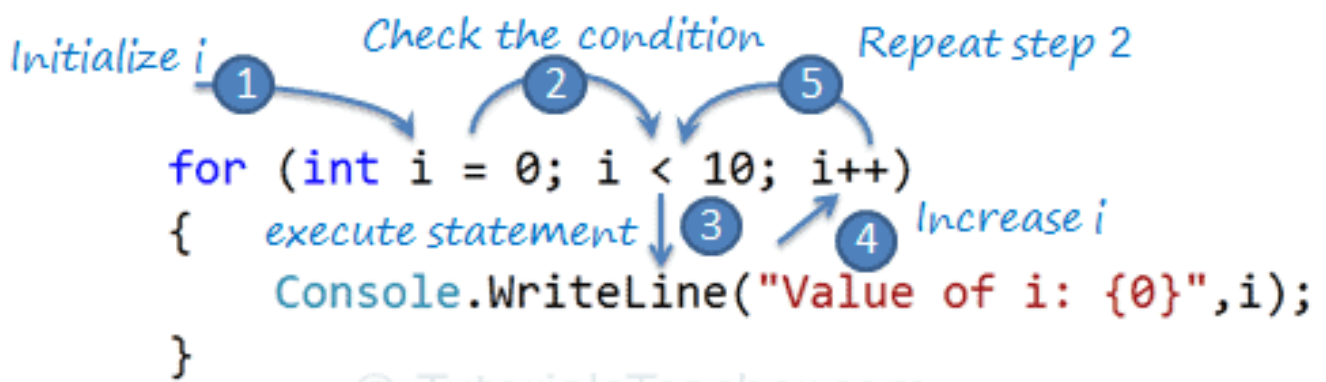
for Loop Execution Steps
